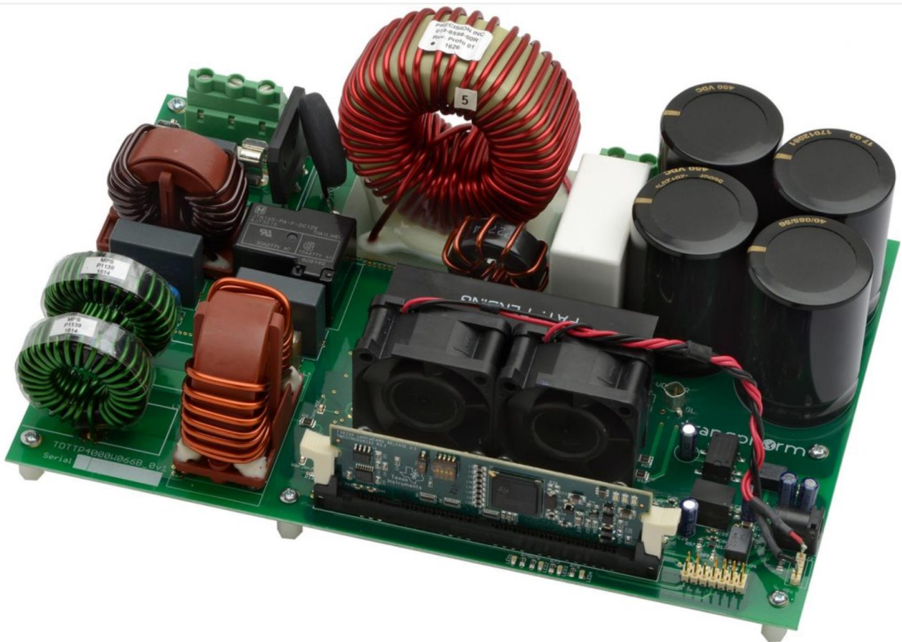
Figure 1. TDTP4000W066B 4kW bridge-less totem-pole PFC evaluation board
